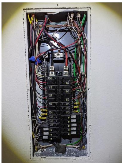
Secondary Panel Wiring
